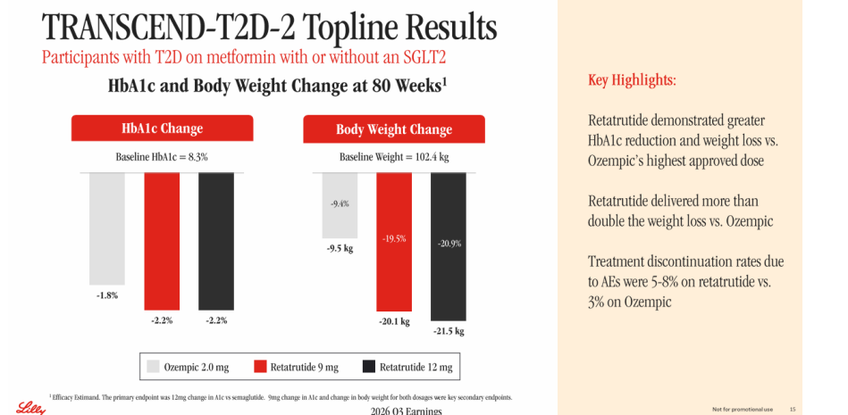
Figure 8: LLY Pipeline
