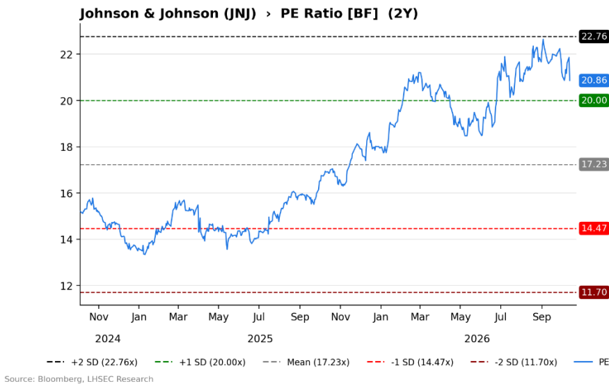
Figure 4: Blended Forward PER
